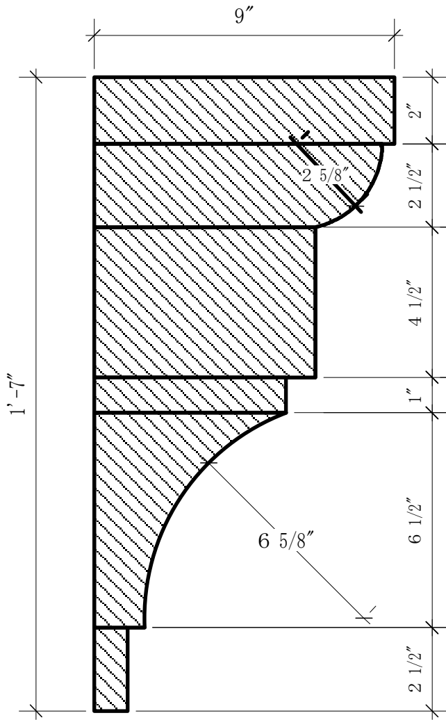
PARTY PORTAL CROWN MOLDING PROFILE
